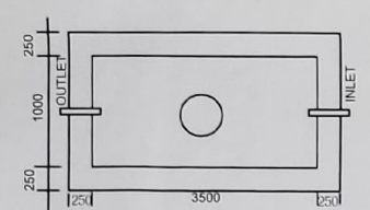
PLAN. SCALE-1:50. SEMI-UNDERGROUND WATER RESERV.
