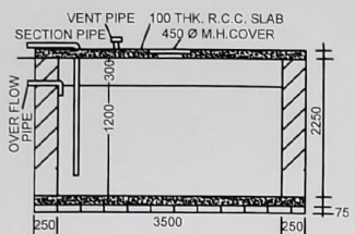
SECTIONAL ELEVATION
