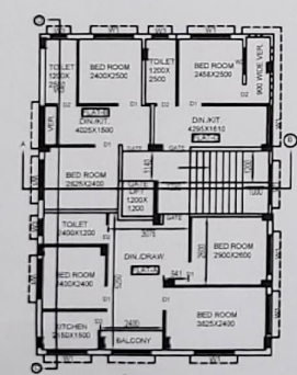
TYPICAL FLOOR PLAN SCALE:1:100
