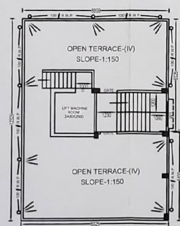
ROOF PLAN SCALE:1:100
